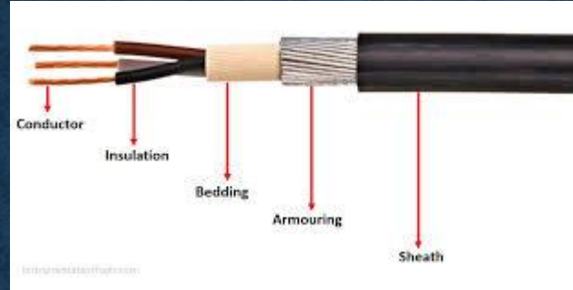
Armoured Cables
